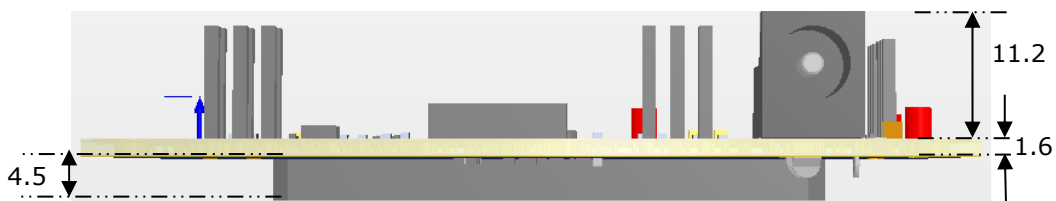
Figure 2-6 UMFT600A/UMFT601A Dimensions (Side view)
